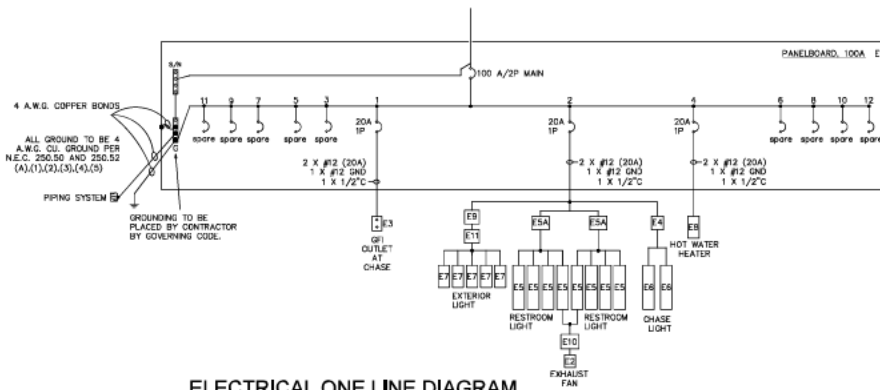
ELECTRICAL ONE LINE DIAGRAM
