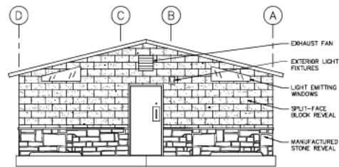
3 REAR ELEVATION SCALE: 1/4" = 1'-0"
