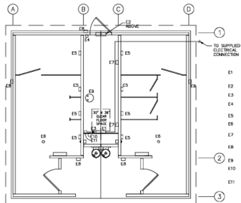
MODULE A MODULE B PLAN VIEW ELECTRICAL SCALE: 1/4" = 1'-0"
