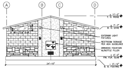
1 FRONT ELEVATION SCALE: 1/4" = 1'-0"
