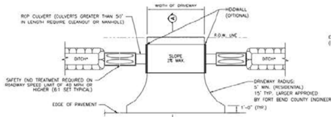
OPEN DITCH DRIVEWAY
