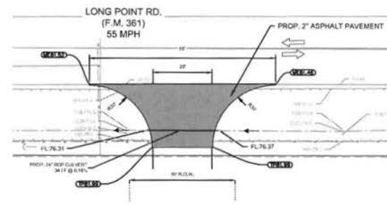
DRIVEWAY DETAILS
