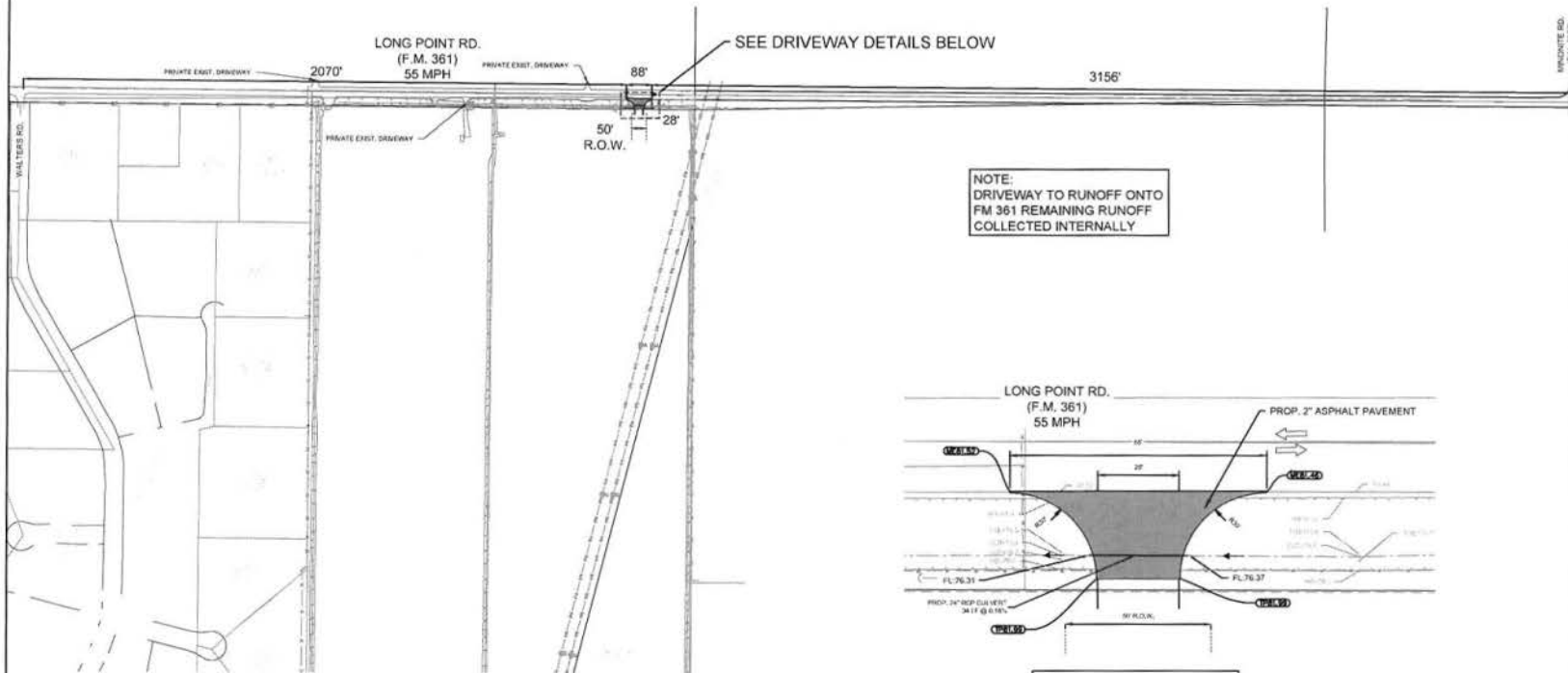
DRIVEWAY DETAILS
