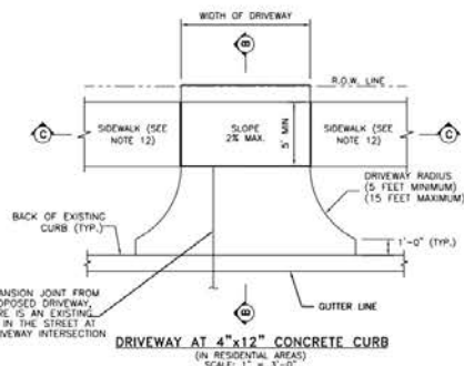
DRIVEWAY AT 4"x12" CONCRETE CURB (IN RESIDENTIAL AREAS) SCALE: 1" = 3'-0"
