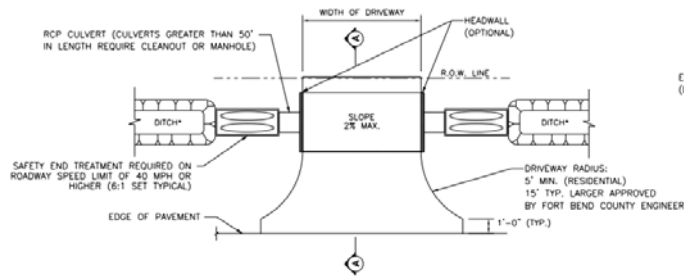
OPEN DITCH DRIVEWAY
