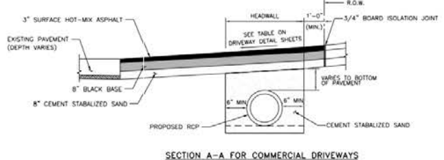
SECTION A-A FOR COMMERCIAL DRIVEWAYS
