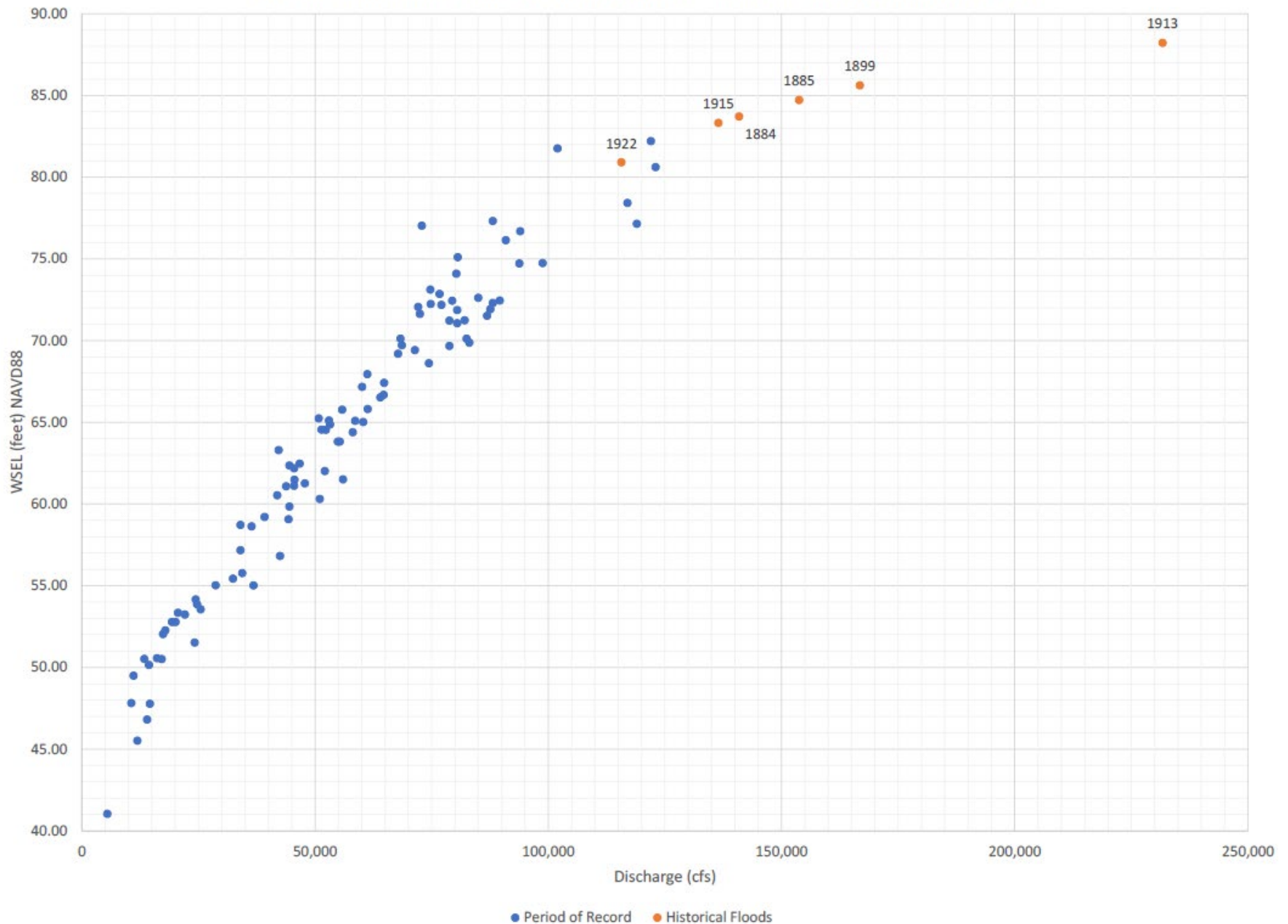
Figure 12. WSEL vs Discharges for Period of Record (1922-2019) and Historical Floods
