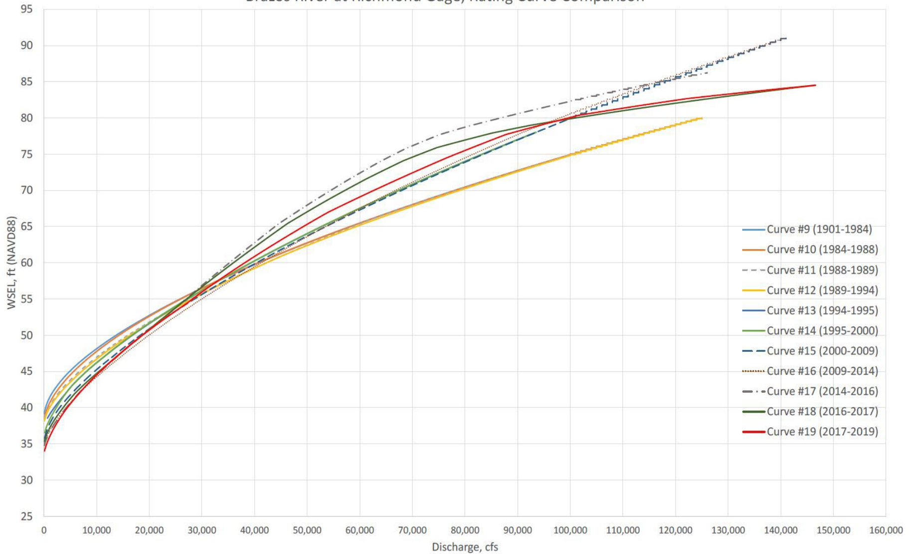
Brazos River at Richmond Gage, Rating Curve Comparison
