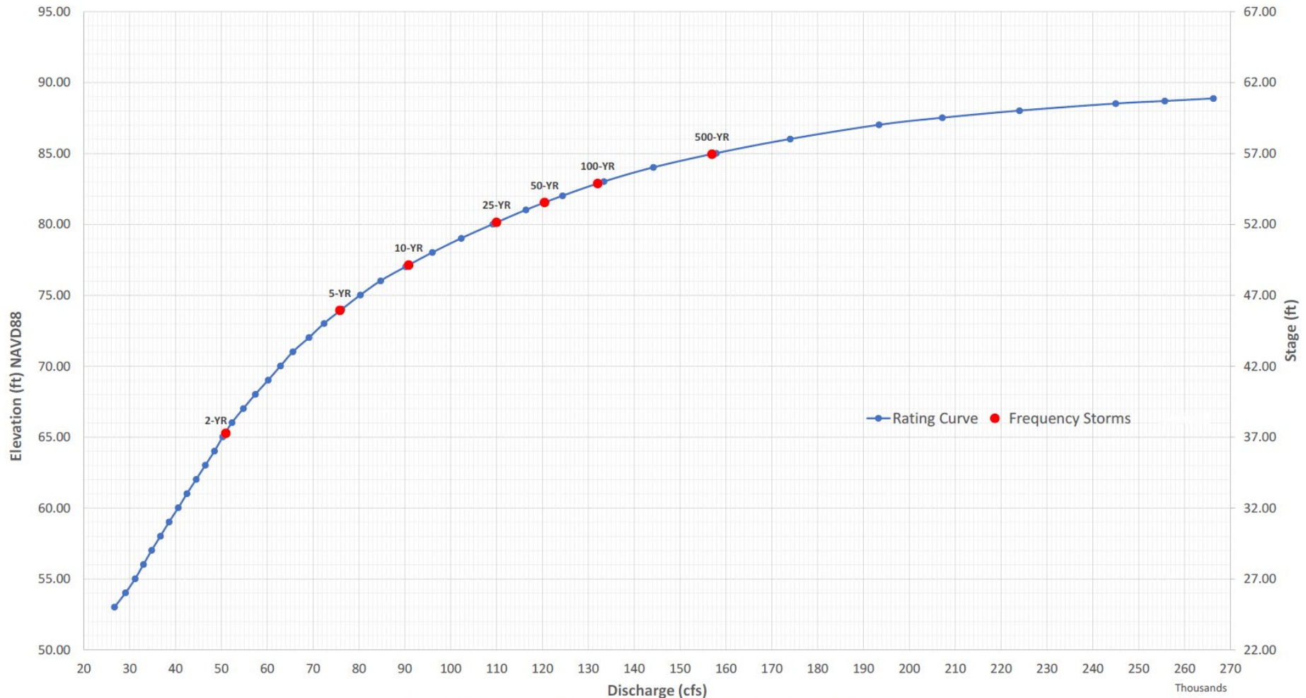
Figure 10. Brazos River at Richmond Gage, Discharge Rating Curve from 1D/2D Model
