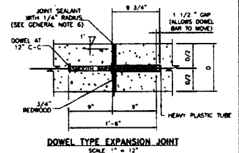
DOWEL TYPE EXPANSION JOINT SCALE: 1" = 12"
