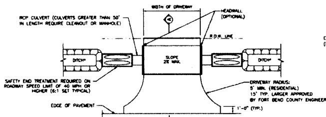
OPEN DITCH DRIVEWAY
