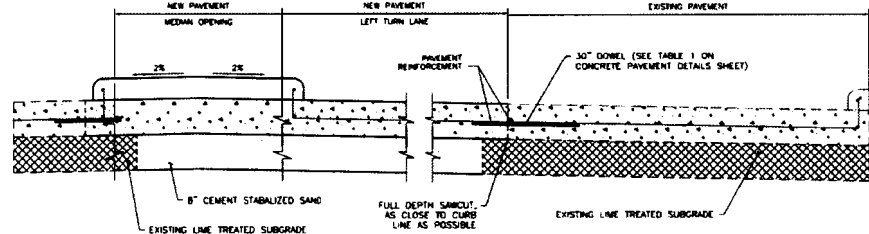
LEFT TURN LANE & MEDIAN OPENING
