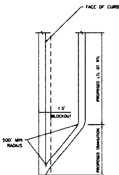
TURN LANE PLAN VIEW
