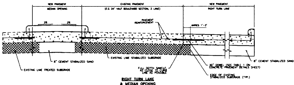
RIGHT TURN LANE & MEDIAN OPENING
