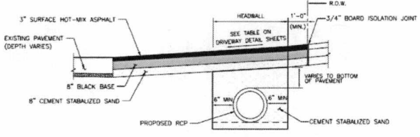
SECTION A-A FOR COMMERCIAL DRIVEWAYS
