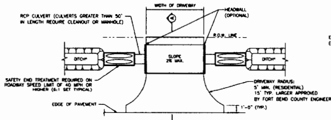
OPEN DITCH DRIVEWAY WIDTH IS TO HAVE 4:1 SLOPE
