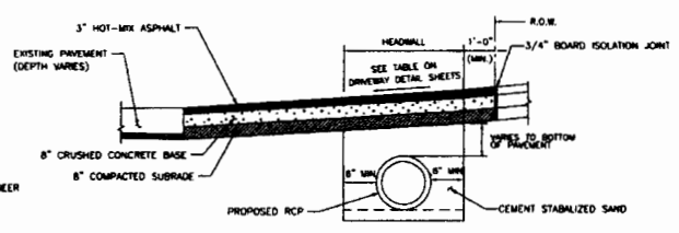
SECTION A-A FOR RESIDENTIAL DRIVEWAYS
