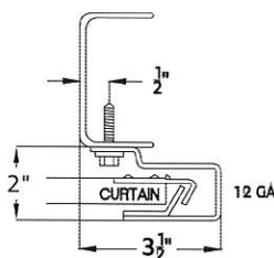
Guide Detail Mount to Steel
