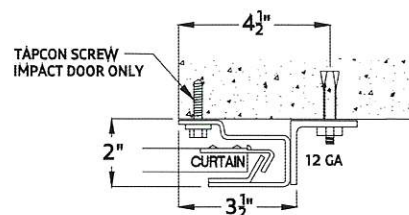
Guide Detail Mount to Masonry
