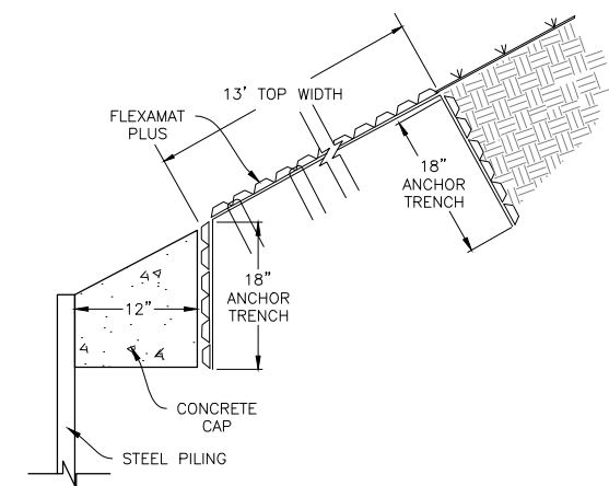
FLEXMAT SECTION VIEW
