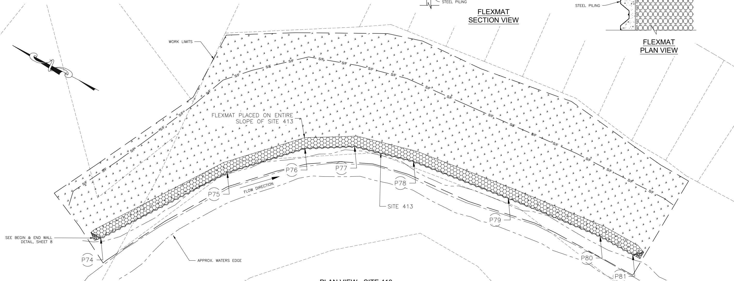
PLAN VIEW - SITE 413
