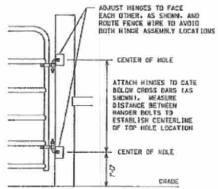
DETAIL "B" GATE POST HINGE ATTACHMENT DETAIL
