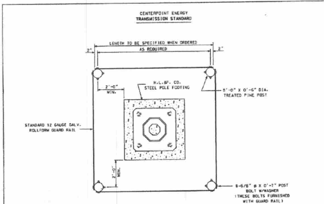
PLAN
