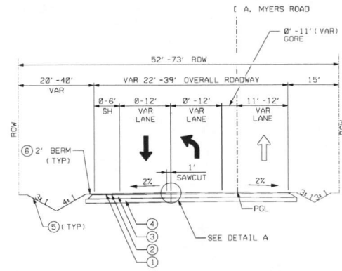
PROPOSED TYPICAL SECTION STA 16+25.85 TO STA 22+88.58
