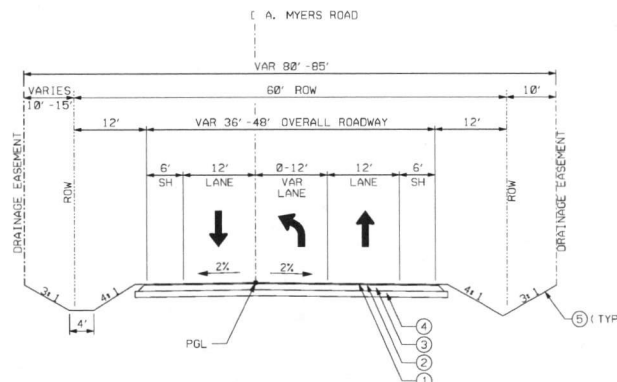
PROPOSED TYPICAL SECTION STA 85+32.62 TO STA 88+88.23
