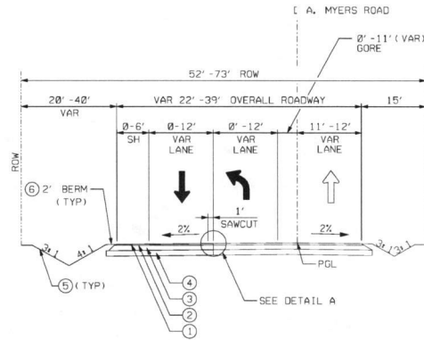
PROPOSED TYPICAL SECTION STA 16+25.85 TO STA 22+80.50
