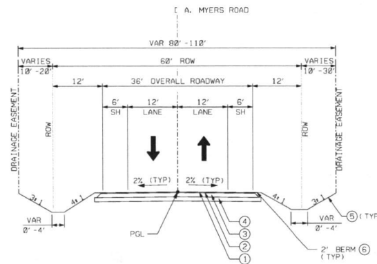
PROPOSED TYPICAL SECTION STA 26+54.04 TO STA 85+32.62
