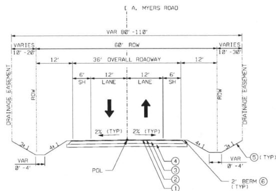
PROPOSED TYPICAL SECTION STA 26+54.84 TO STA 85+32.62
