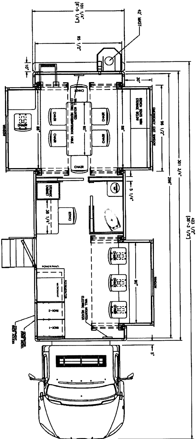
FLOOR PLAN VIEW
