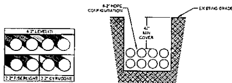
TYPICAL DETAIL "D" HDPE CONFIGURATION
