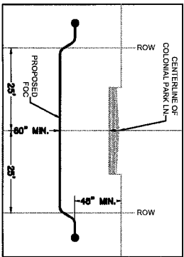
SHEET 52 BORE PROFILE LOOKING NORTH COLONIAL PARK LN.
