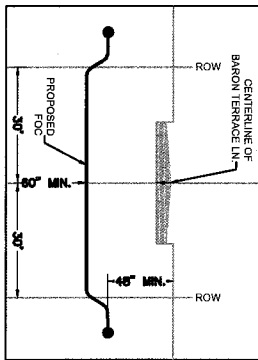
SHEET 50 BORE PROFILE LOOKING NORTH BARON TERRACE LN.
