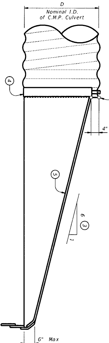
SIDE ELEVATION OF END SECTION
