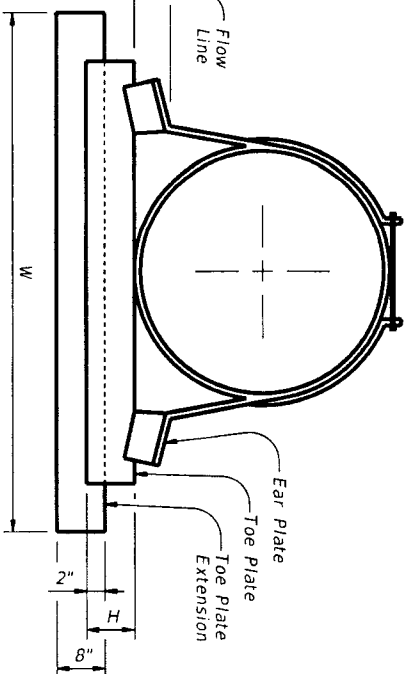
END ELEVATION OF END SECTION
