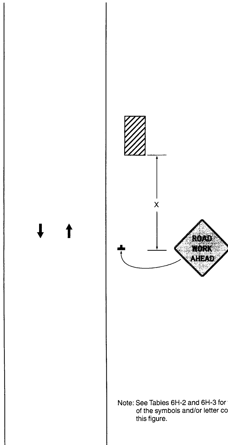
Typical Application 1
