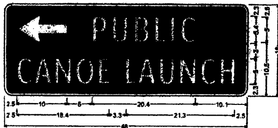
D7-5L; 1.5" Radius, 0.5" Border, White on Brown; Standard Arrow Custom 10.0" X 5.4" 180°; "PUBLIC" ClearviewHwy-2-W; "CANOE LAUNCH" ClearviewHwy-2-W 70% spacing.
