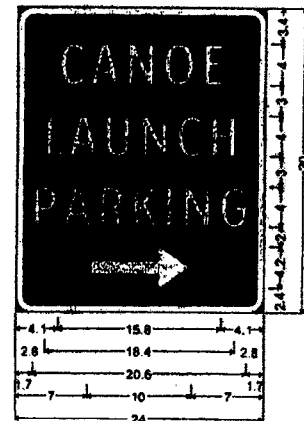
1.5" Radius, 0.8" Border, White on Brown; "CANOE" ClearviewHwy-2-W; "LAUNCH" ClearviewHwy-2-W; "PARKING" ClearviewHwy-2-W; Standard Arrow Custom 10.0" X 4.1" 0°;
