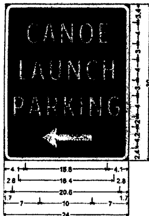
1.5" Radius, 0.8" Border, White on Brown; "CANOE" ClearviewHwy-2-W; "LAUNCH" ClearviewHwy-2-W; "PARKING" ClearviewHwy-2-W; Standard Arrow Custom 10.0" X 4.1" 180°;
