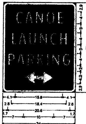
1.5" Radius, 0.8" Border, White on Brown; "CANOE" ClearviewHwy-2-W; "LAUNCH" ClearviewHwy-2-W; "PARKING" ClearviewHwy-2-W; Double Arrow;
