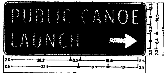
D7-5L; 1.5" Radius, 0.5" Border, White on Brown; "PUBLIC CANOE" ClearviewHwy-2-W specified length; "LAUNCH" ClearviewHwy-2-W, Standard Arrow Custom 10.0" X 5.4" 0°;
