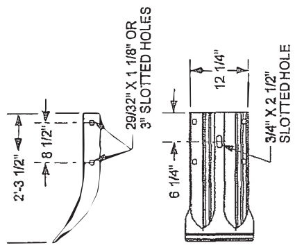
12 GAGE END SECTION
