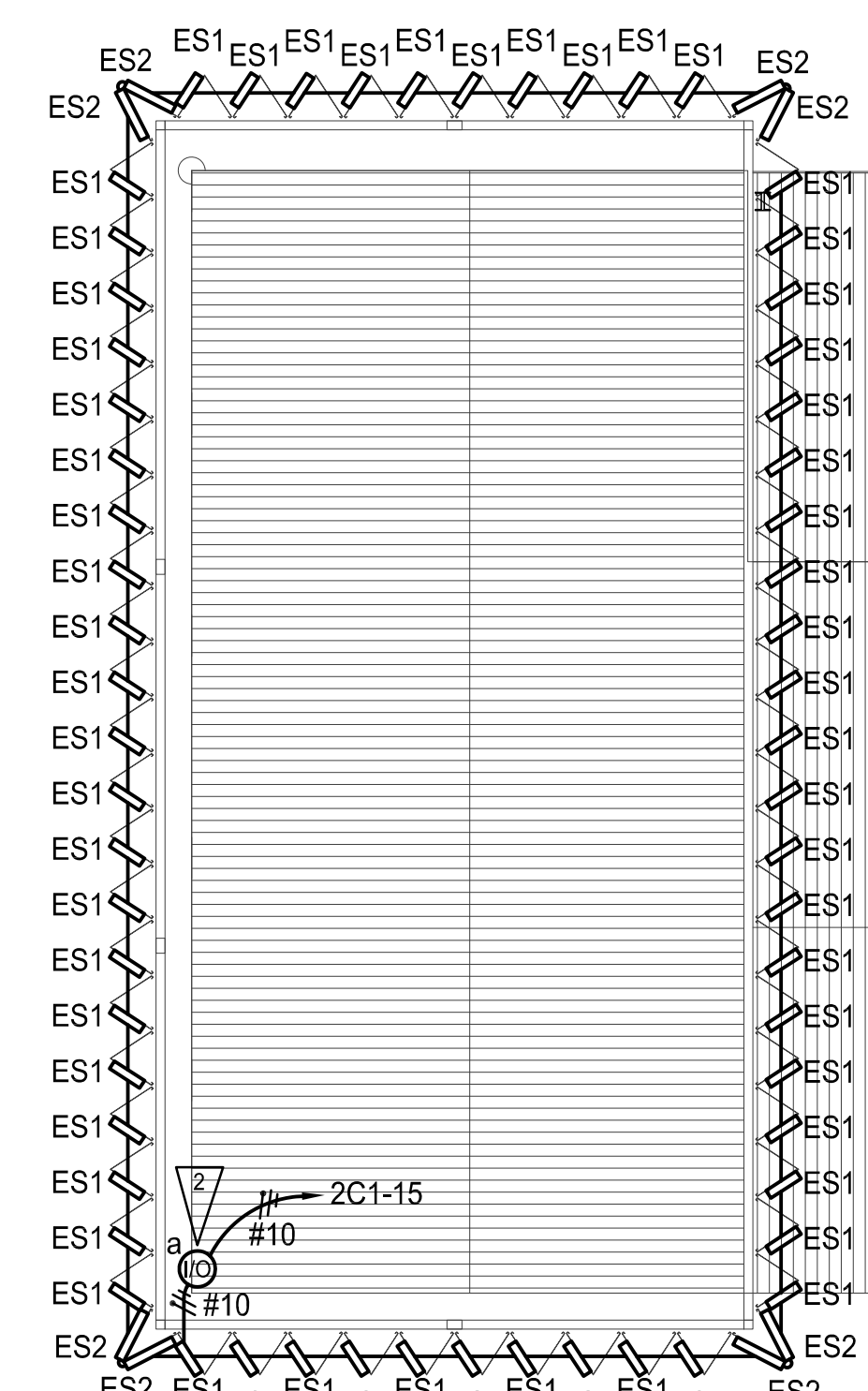
CROWN LIGHTING PLAN SCALE: 1"=10'-0"
