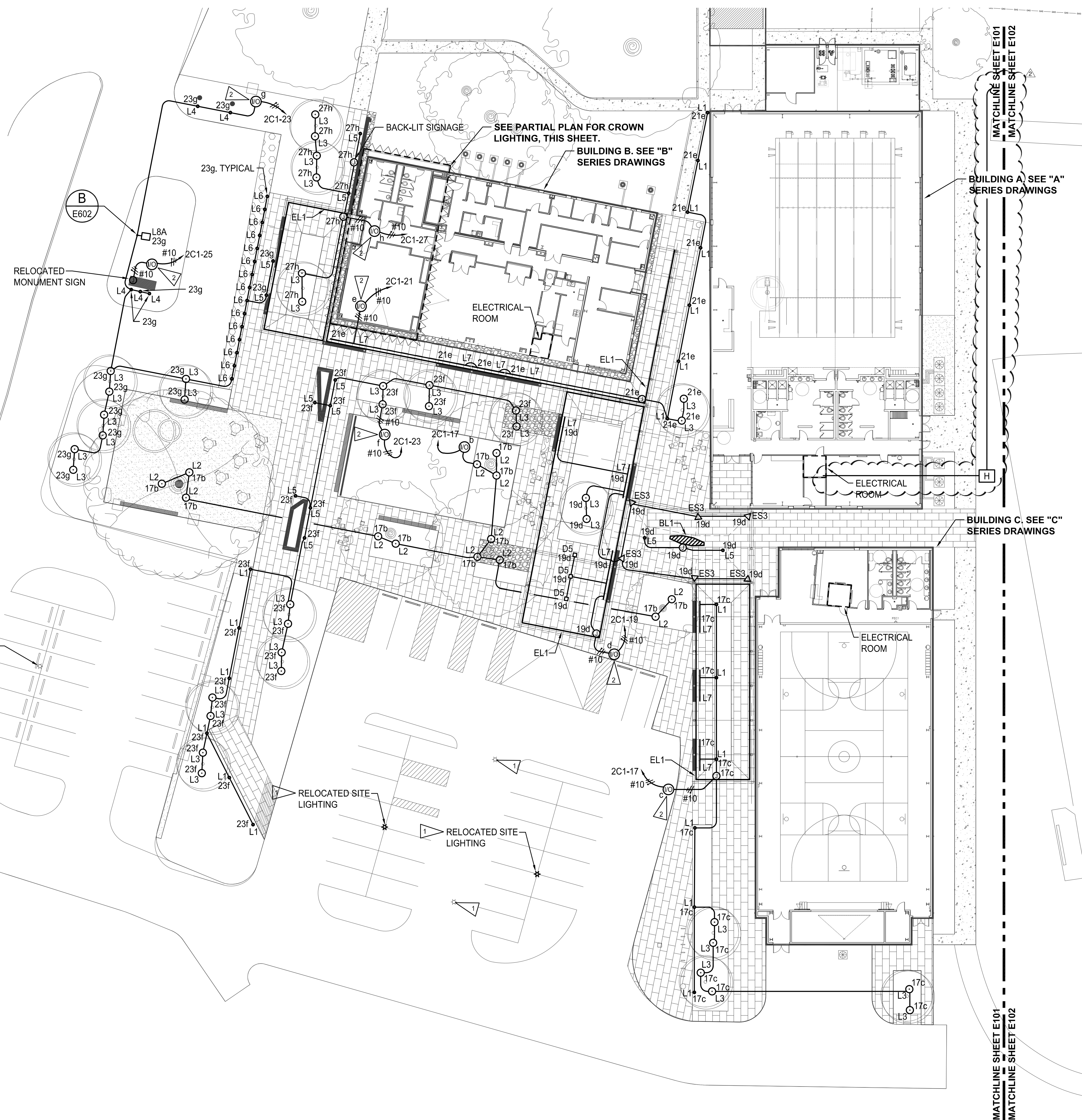
ELECTRICAL SITE LIGHTING PLAN SCALE: 1"=20'-0"
