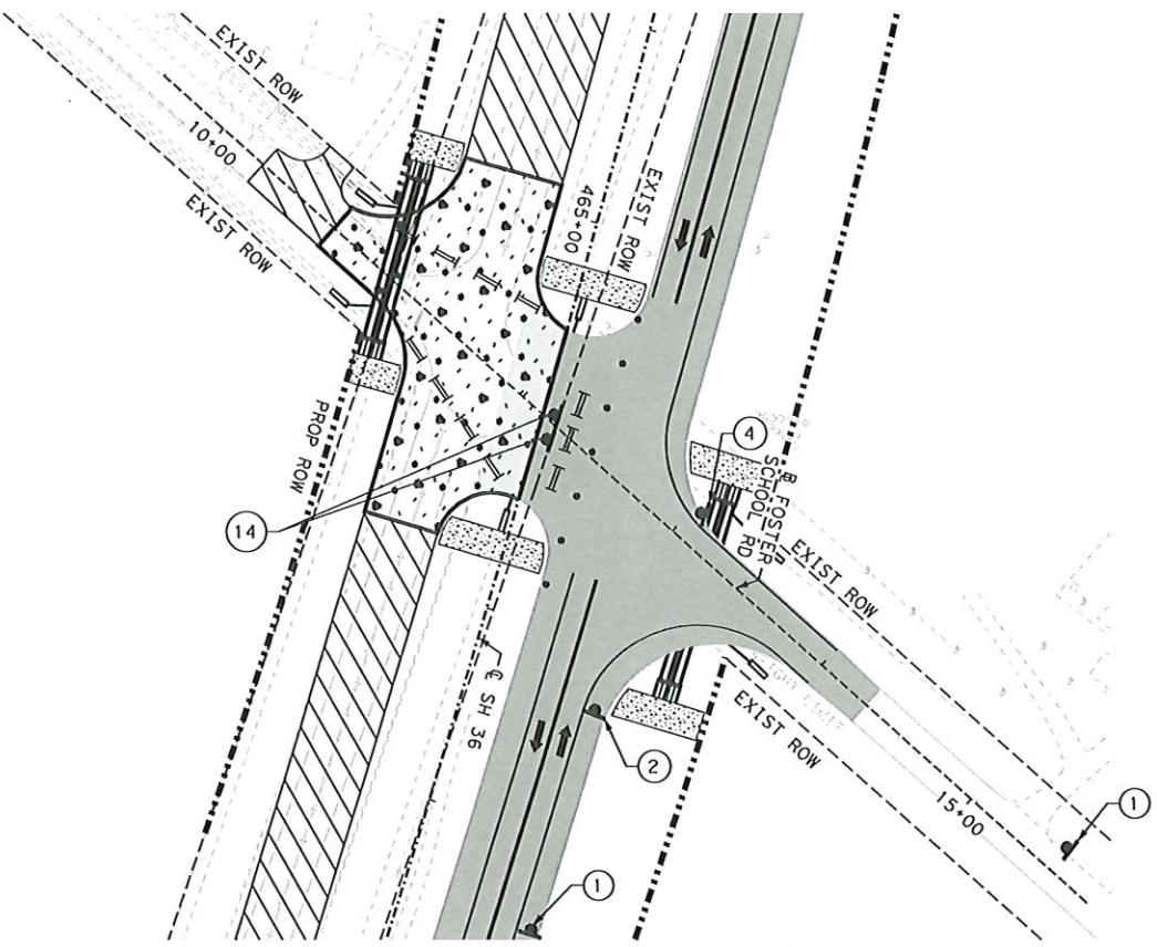
DETAIL A-A SCALE IN FEET 0' 50' 100'
