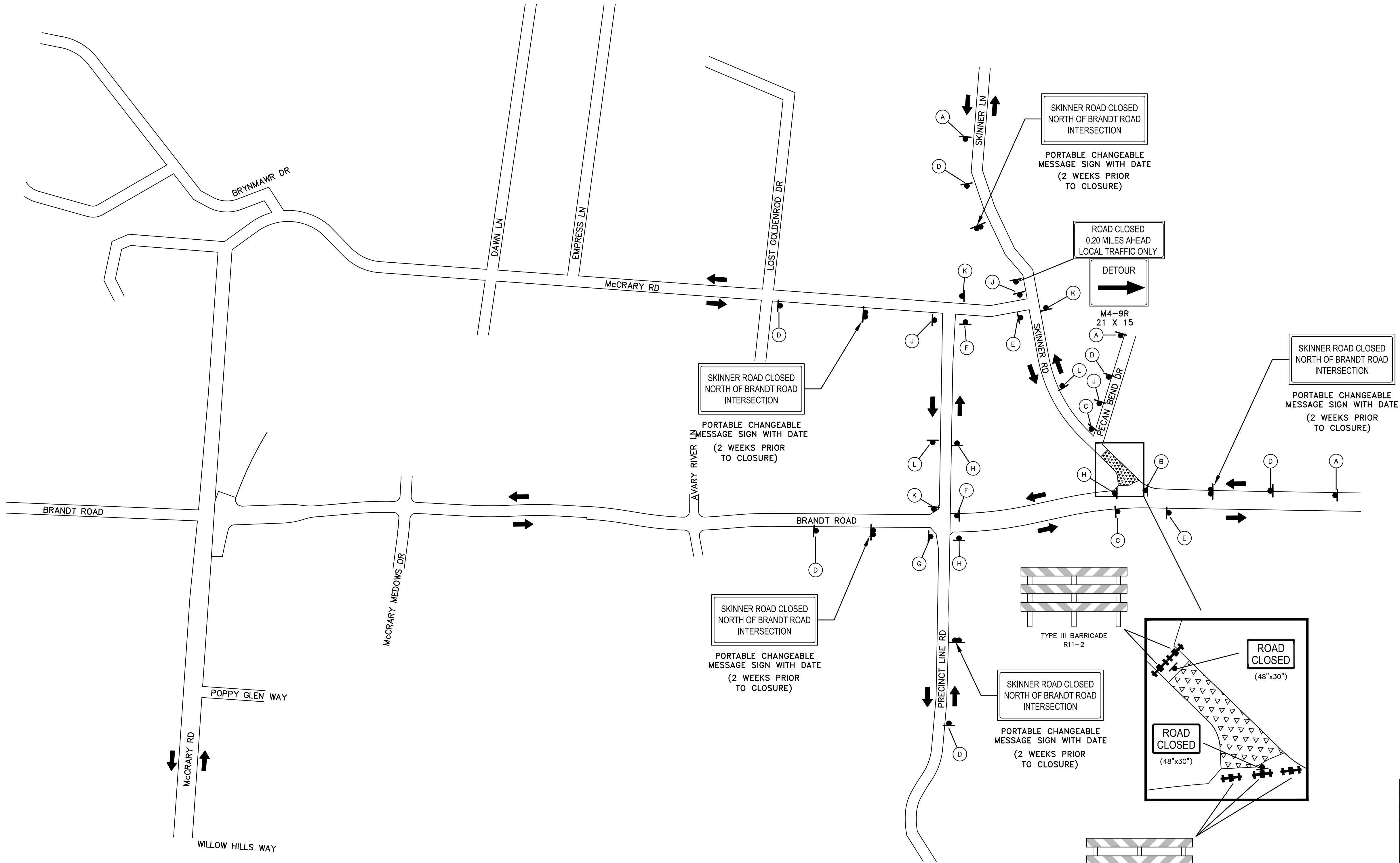
TRAFFIC CONTROL PLAN PHASE 1 – STEP 3 © BRANDT ROAD AND SKINNER RD DETOUR PLAN
