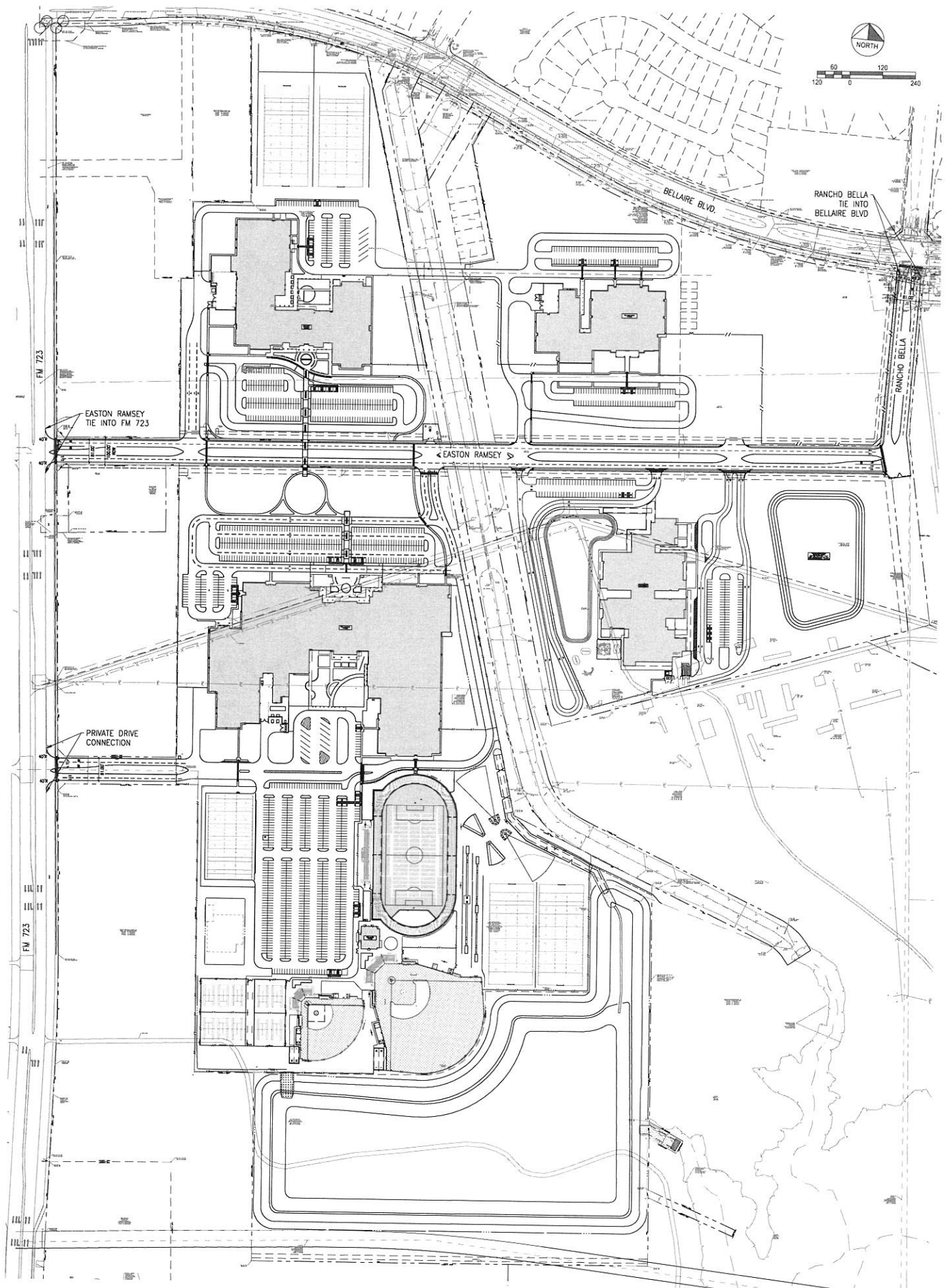
STREET TIE IN FOR LAMAR CONSOLIDATED CAMPUS COMPLEX SEC 1 EXHIBIT
