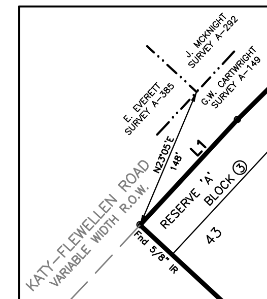
SURVEY TIE DETAIL SCALE: 1"=100'
