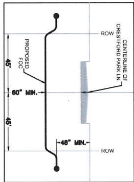
SHEET 57 BORE PROFILE LOOKING NORTH CRESTFORD PARK LN.
