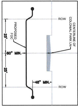
SHEET 52 BORE PROFILE LOOKING NORTH COLONIAL PARK LN.
