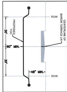
SHEET 50 BORE PROFILE LOOKING NORTH BARON TERRACE LN.
