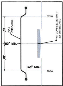
SHEET 51 BORE PROFILE LOOKING NORTH ADDISON HILLS LN.
